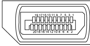
Figure 6. DisplayPort (out)
