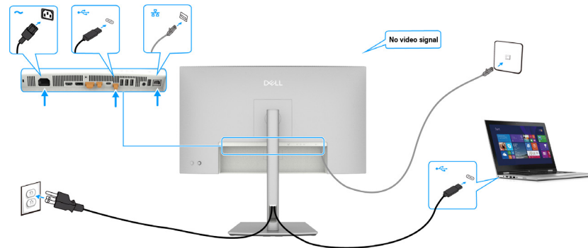
Figure 38. Network routing via USB-C upstream port
